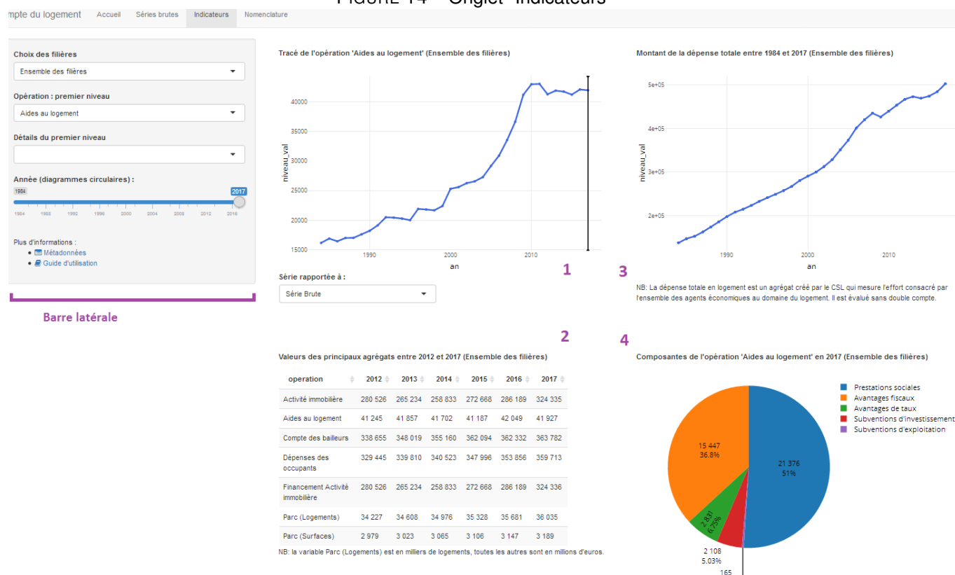
FIGURE 14 – Onglet "Indicateurs"
