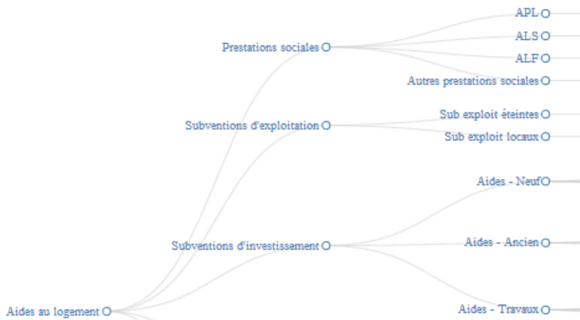
FIGURE 16 – Nomenclature "Aides"
